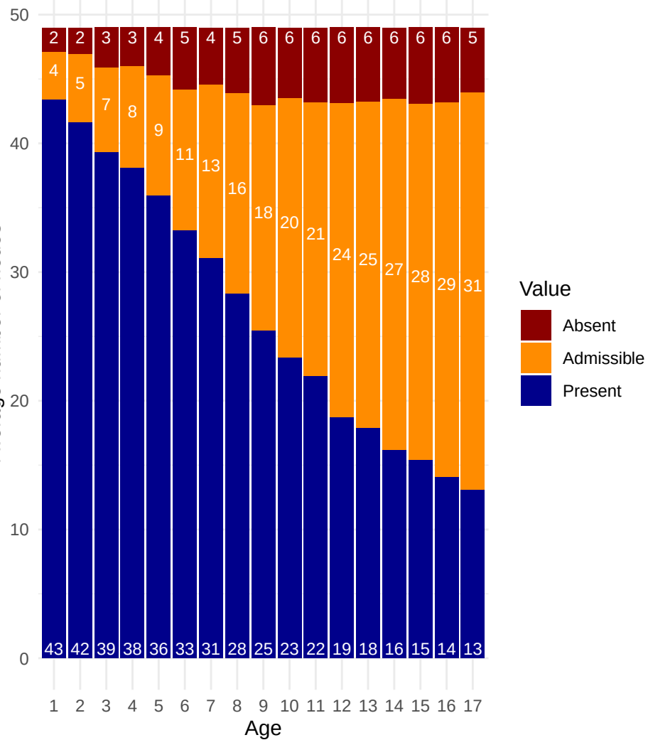
Consensus
