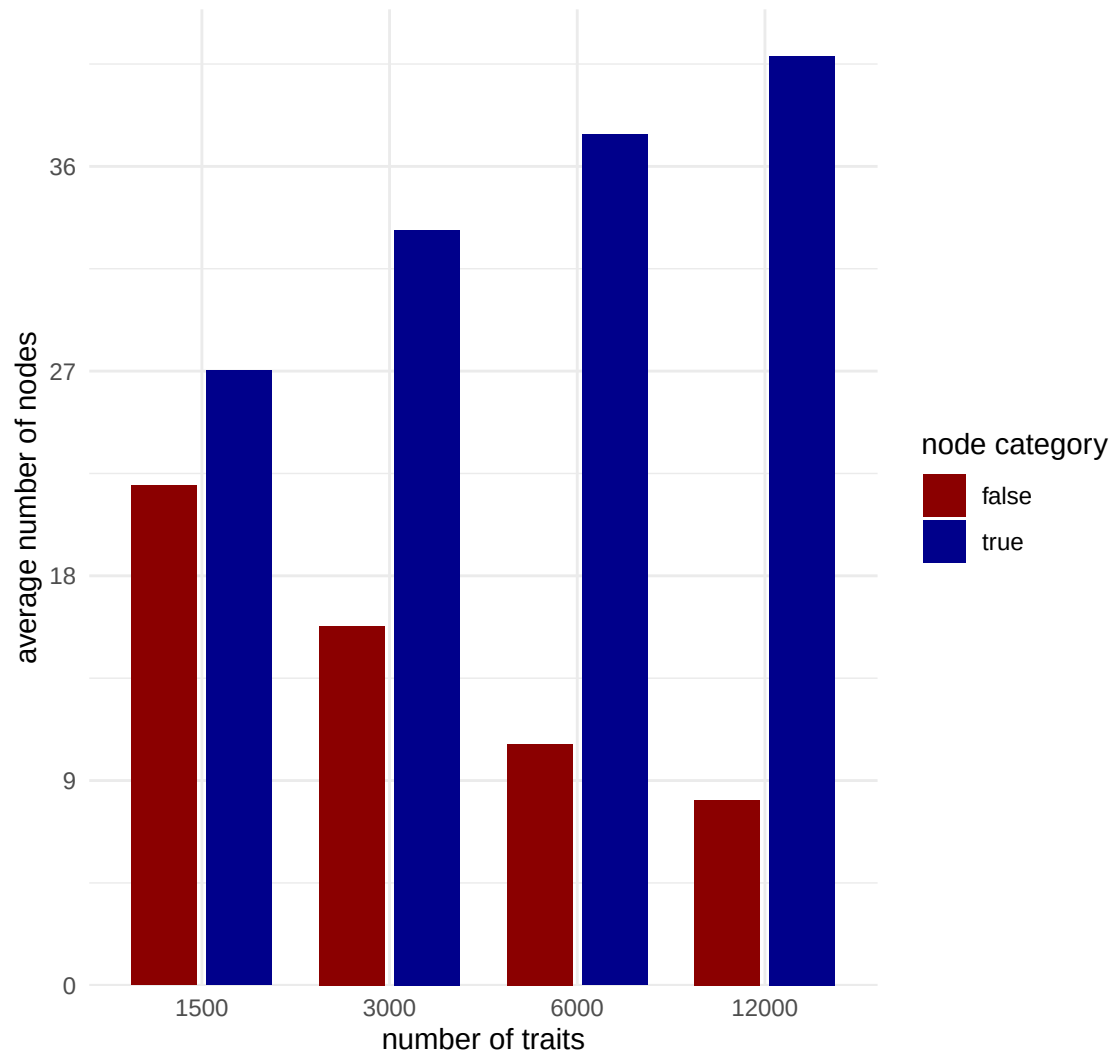
MCC
