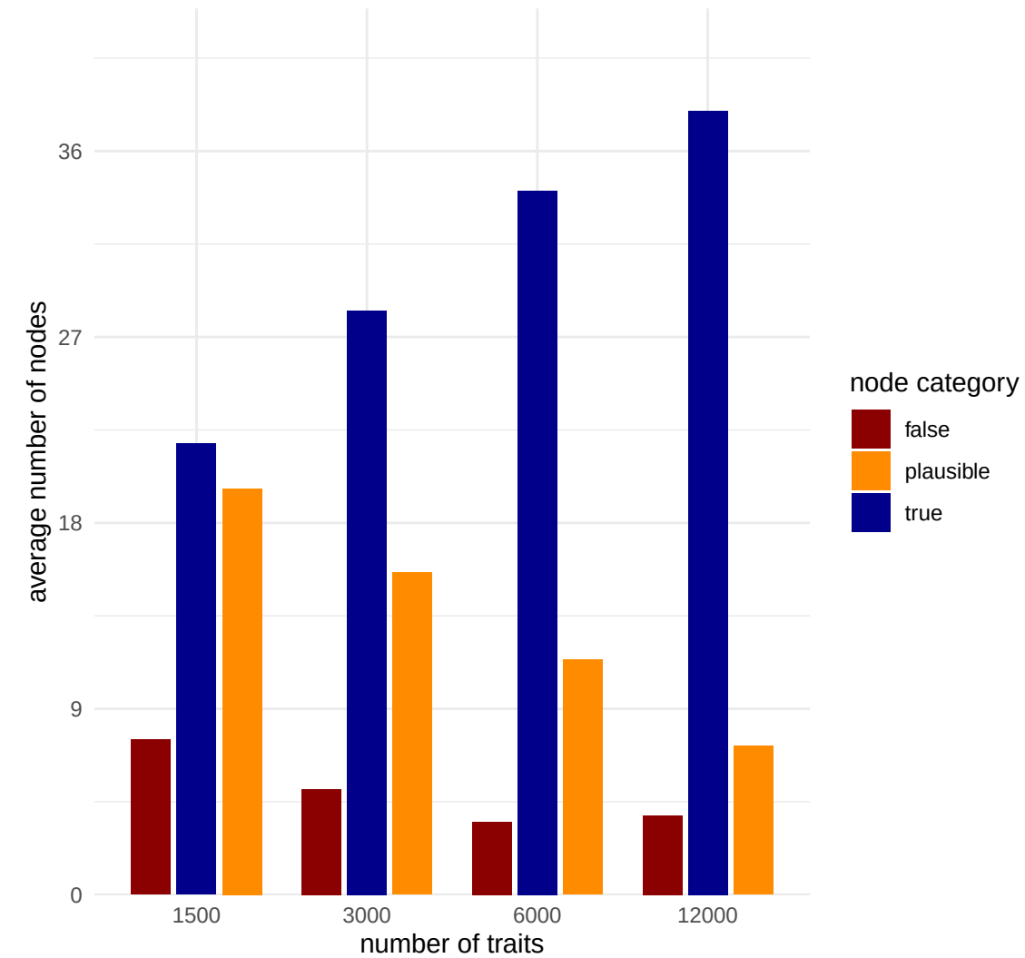
Consensus
