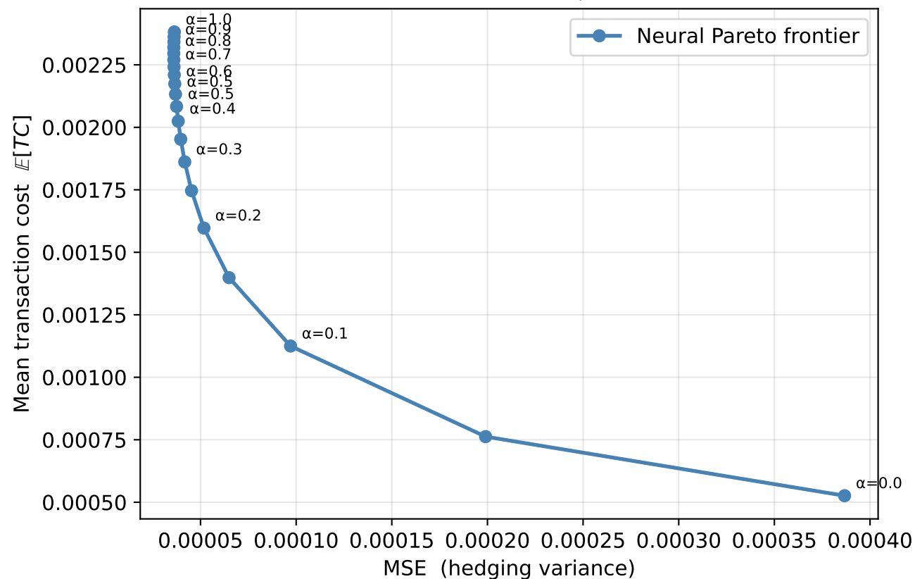
Figure 12 — Pareto frontier: risk vs cost GBM call · c=0.02 , l=0.2
