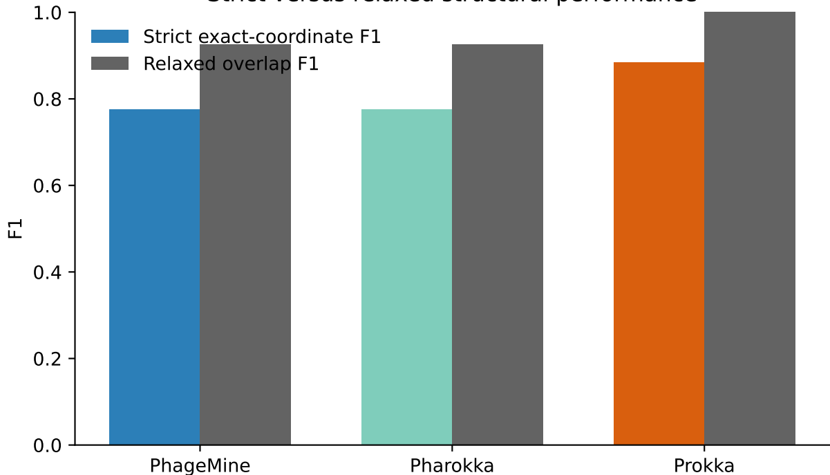
Strict versus relaxed structural performance
