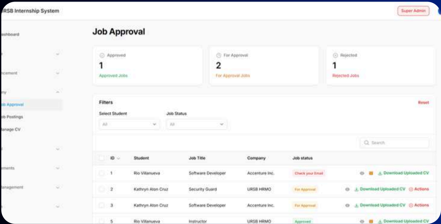
Job Approval
