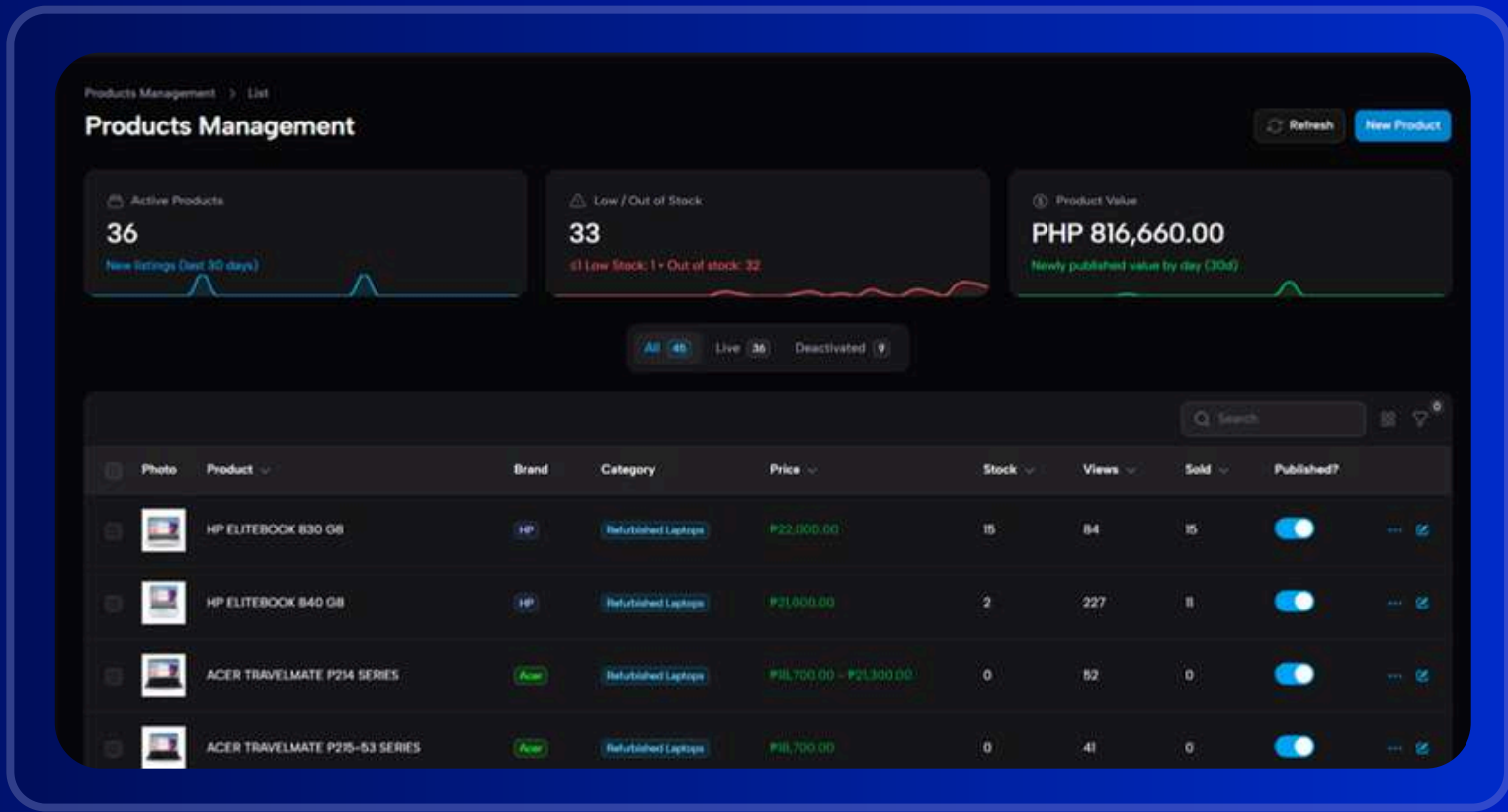
Products Management
