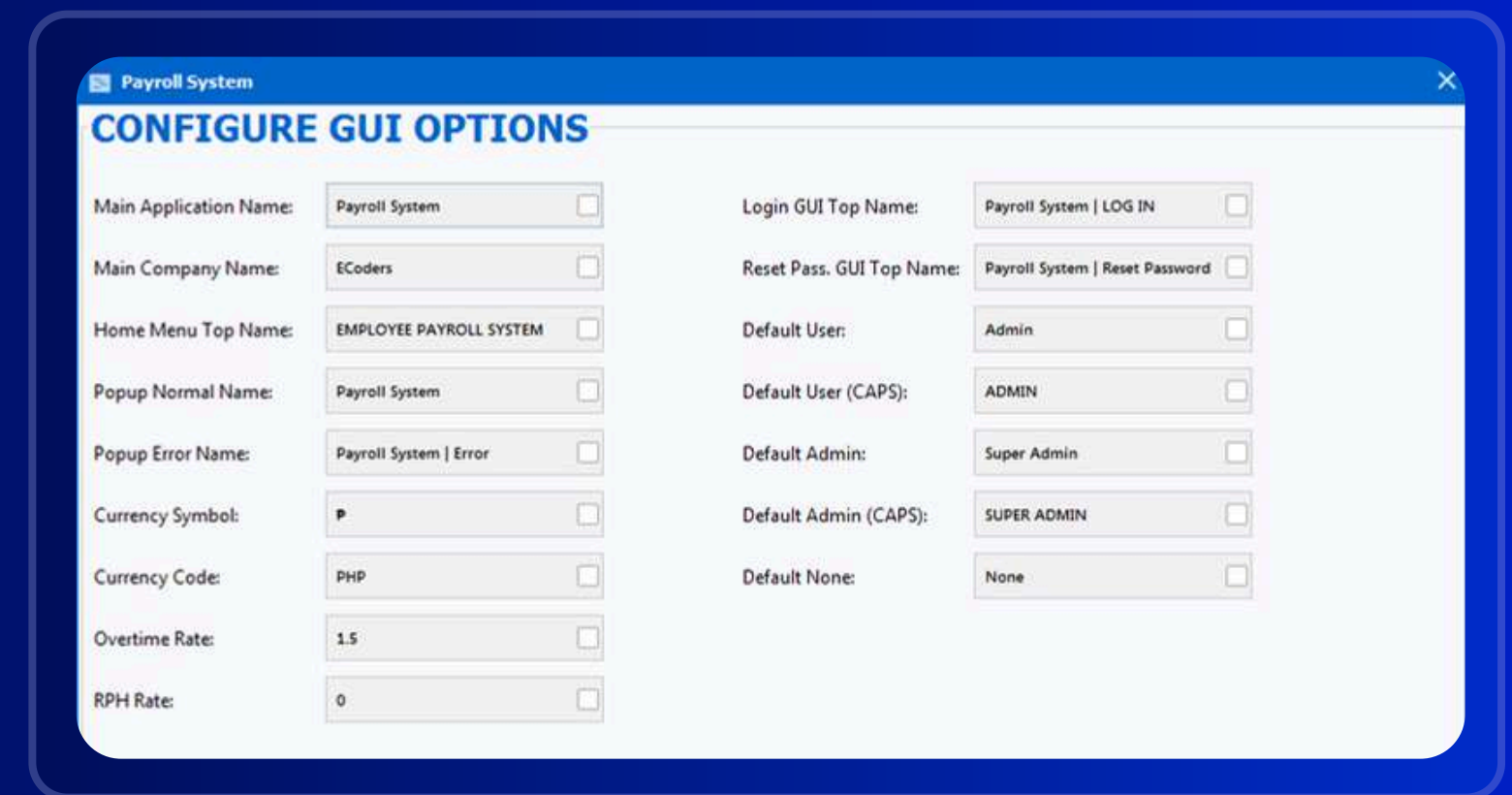
GUI Configuration
