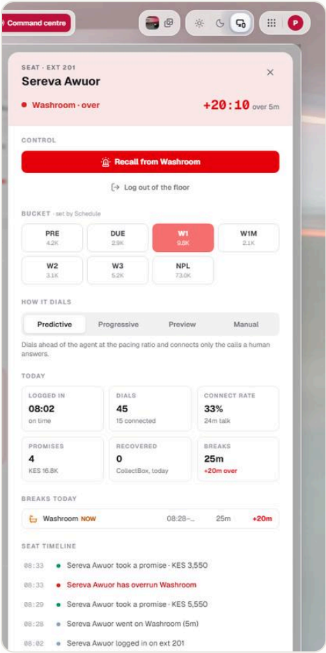
The seat drawer for an agent 20 minutes over a washroom break.
