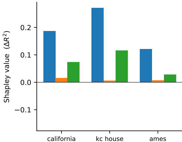
uniform standardisation
