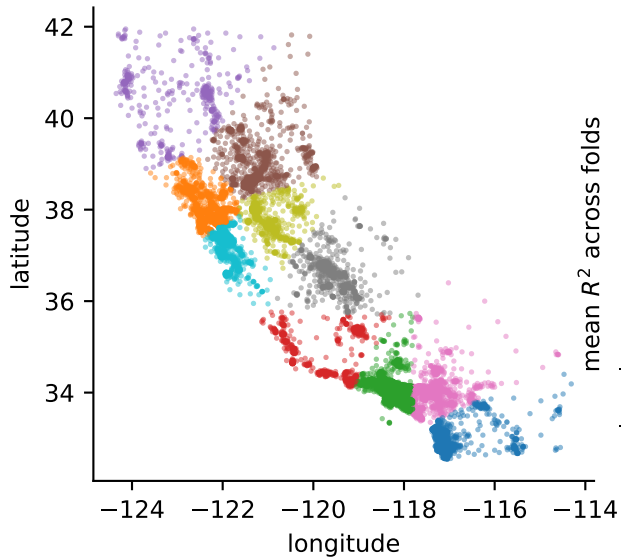
spatial blocks used as CV folds
