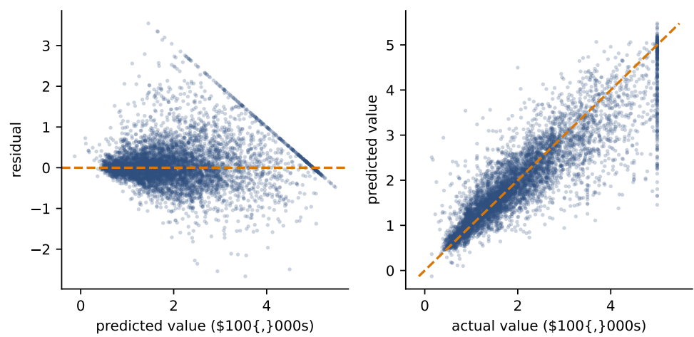
Fig. 8 Residuals against predicted values (left) and actual against predicted values (right) for the final configuration on the held-out test set. The vertical band of true values at 5.0 in the right panel is the census recording cap.
