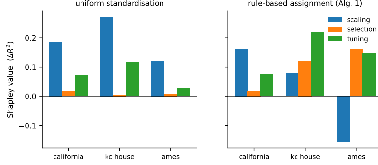
Fig. 6 Shapley attribution of the three workflow components on each dataset, under uniform standardisation (left) and under the distribution-aware scaler rule of Algorithm 1 (right). Under uniform standardisation the ordering scaling > tuning > selection is preserved on all three datasets; under the rule it is not, and on Ames the scaling contribution is negative.
