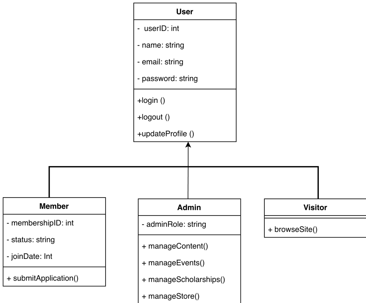
Class Diagram
