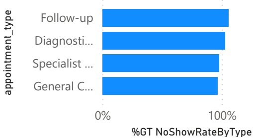
appointment_type
