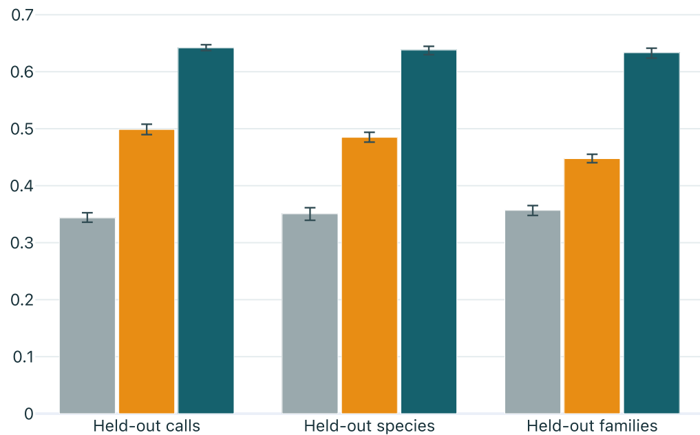
Cosine similarity ↑
