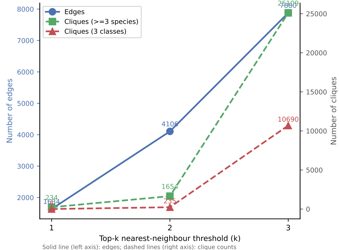
B. SPNN graph sensitivity to top-k threshold
