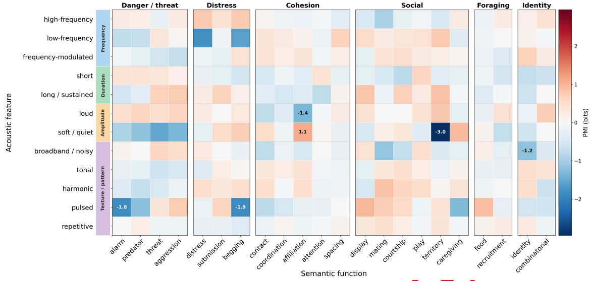
Figure 4. Keyword-level structure of the biological code. Pointwise mutual information (PMI, bits) between semantic functions (columns, grouped into panels by category) and acoustic features (rows, grouped by type), estimated across all 307 calls in AnimalLex. Acoustic features are ordered by group: frequency (high, low, FM), duration (short, long), amplitude (loud, soft), and texture/pattern. Numbers annotate the two strongest and one weakest association per panel. Warm colors = acoustic feature over-represented in calls with that semantic function; cool colors = under-represented.
