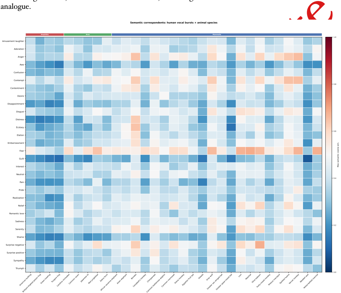
Figure 6. Semantic correspondents between human vocal bursts and animal species. Each cell shows the maximum semantic cosine similarity (L2-normalised sentence embeddings) between a human burst type (row) and any call of an animal species (column). Species are sorted by taxonomic class (Amphibia | Aves | Mammalia, colored bars on top) and alphabetically within class. Annotated cells ( \geq 0.75 ) show the best-matching call name. Warm colors indicate close semantic correspondence.
