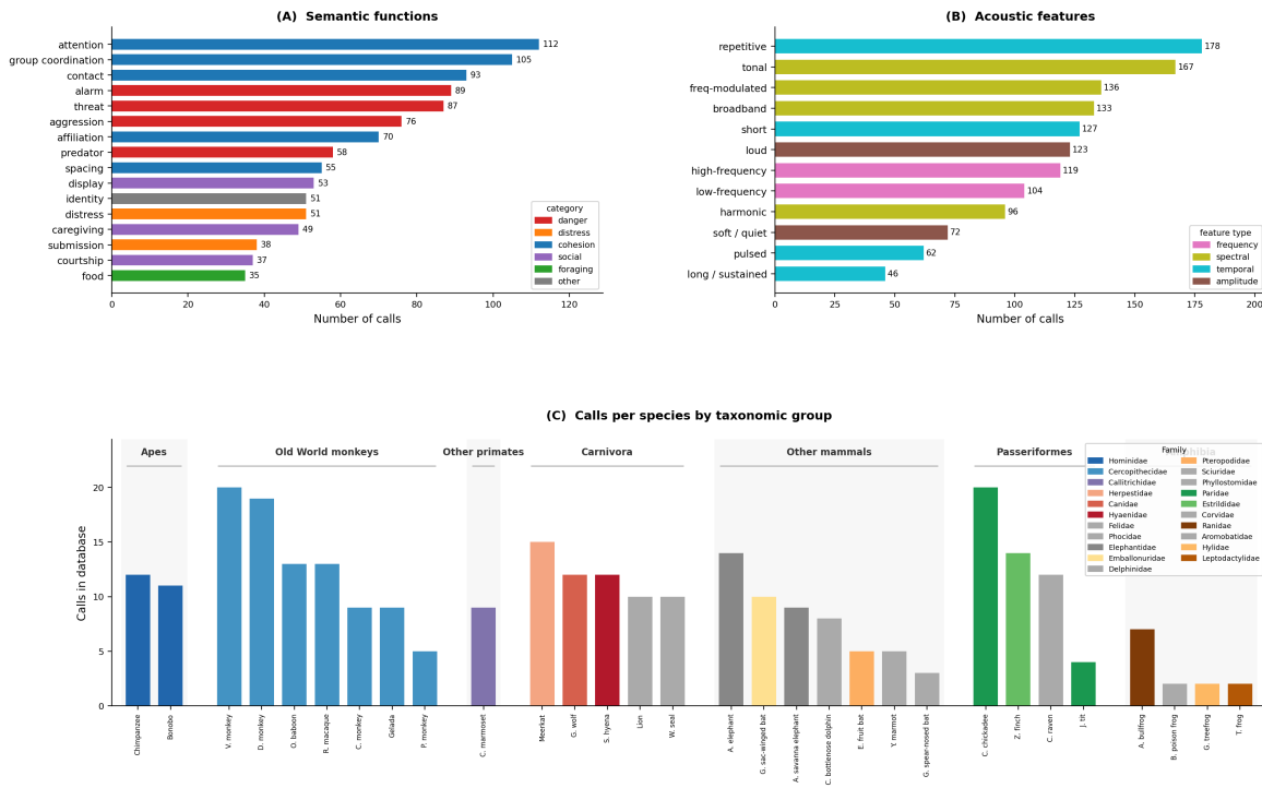
Figure 1. AnimalLex: a curated cross-species lexical repertoire. (A) Frequency of semantic ontology keywords across all 307 calls, colored by communicative category (cohesion, danger, social, distress, foraging, identity/structural). Attention, group coordination, contact, and alarm categories include individual identity and combinatorial structure. (B) Frequency of acoustic features extracted by term-matching from free-text descriptions. Tonal, high-frequency, and repetitive features are most common; soft/quiet and harmonic features are rarer. (C) Calls per species, grouped by taxonomic group (Apes, Old World monkeys, other primates, Carnivora, other mammals, Passeriformes, Psittaciformes, Amphibia) and colored by family. Within each group, species are sorted by repertoire size. Repertoire sizes range from 2 to 20; the largest curated repertoires (20 calls each) are the vervet monkey and the Carolina chickadee.
