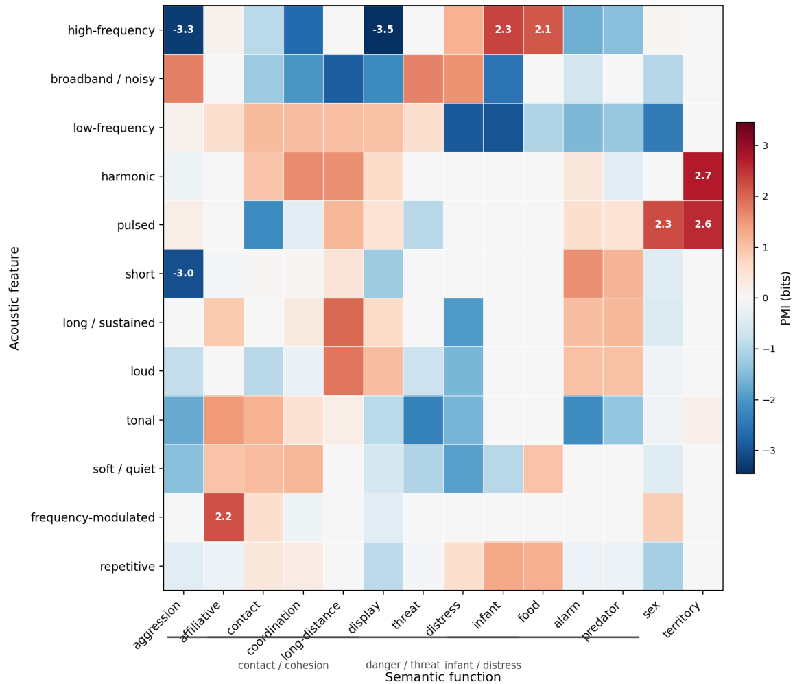
Figure 3. Keyword-level structure of the biological code. Pointwise mutual information (PMI, bits) between acoustic features (rows) and semantic functions (columns), estimated across all 373 calls in AnimalLex. Rows and columns are ordered by hierarchical clustering; numbers annotate the six strongest and three weakest cells. Warm colors = acoustic feature over-represented in calls with that semantic function; cool colors = under-represented. Three groupings are bracketed on the x -axis. Key associations: high-frequency calls are enriched for infant/food contexts (PMI > 2) and depleted for aggression and display (PMI < -3); broadband/noisy calls are enriched for aggression and threat; long/sustained and loud features co-occur with long-distance cohesion calls. These patterns are consistent with functional acoustic ecology predictions and extend them across 57 species.
