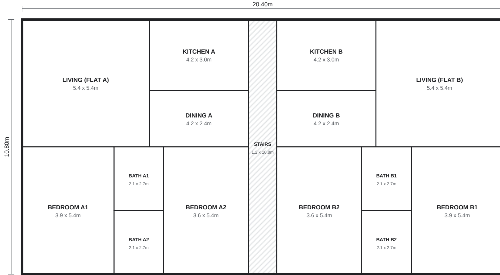
TYPICAL FLOOR PLAN (GROUND AND FIRST FLOOR IDENTICAL) SCALE 1:100
