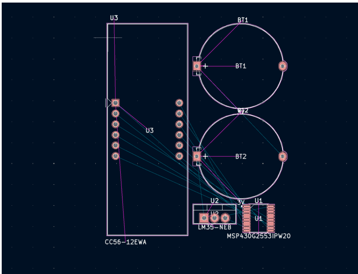
PCB
