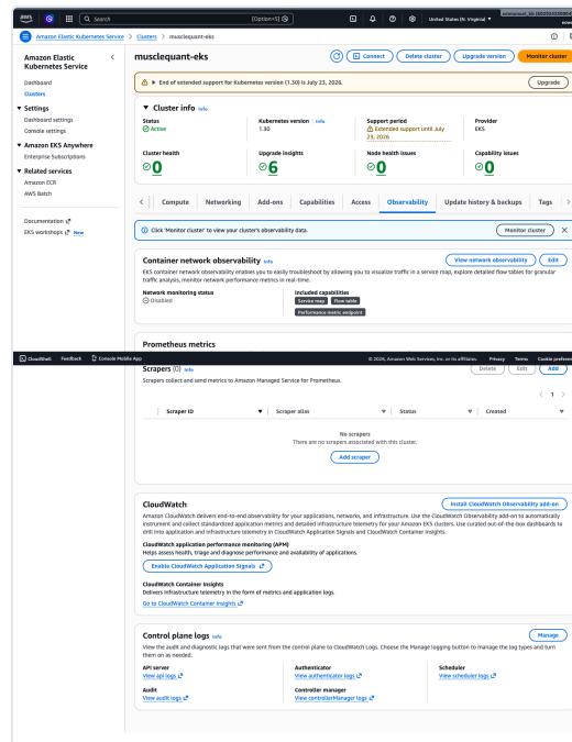
EKS control-plane logging tab in the AWS console
