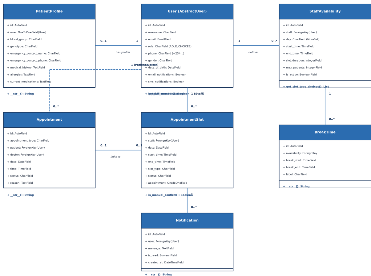
MedSchedule System - Django Domain Class Diagram
