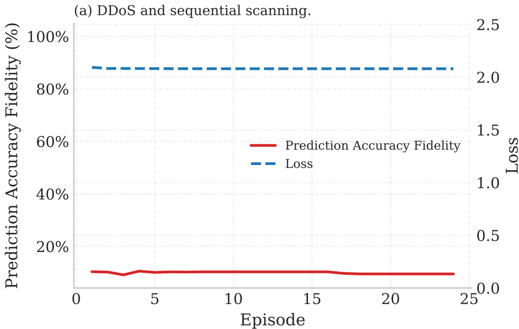
Fig. 7: Prediction accuracy fidelity and loss of attack prediction.
