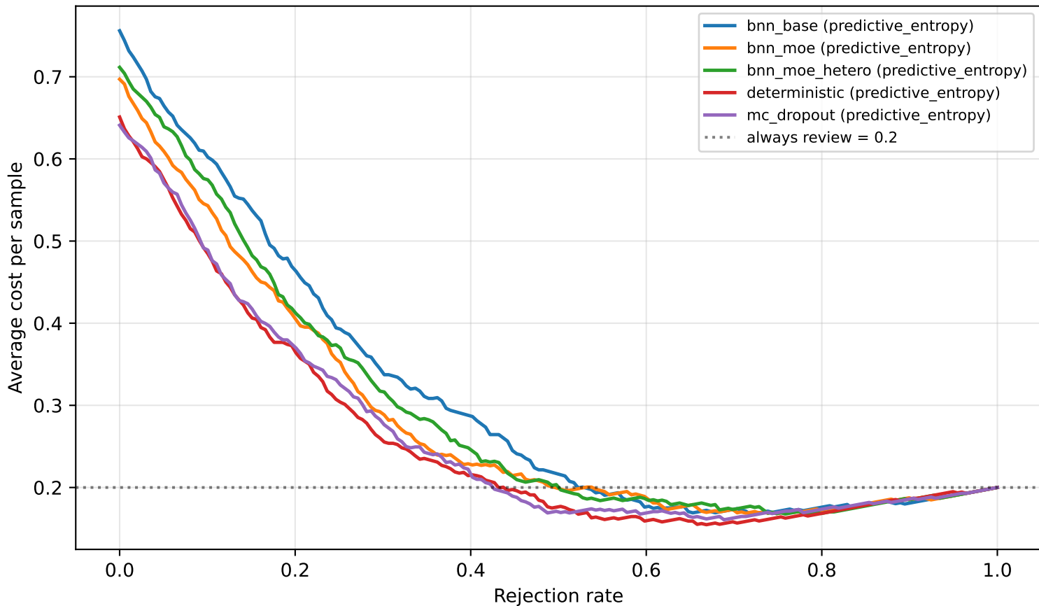
Expected cost vs rejection rate (FP=2.0, FN=5.0, review=0.2)
