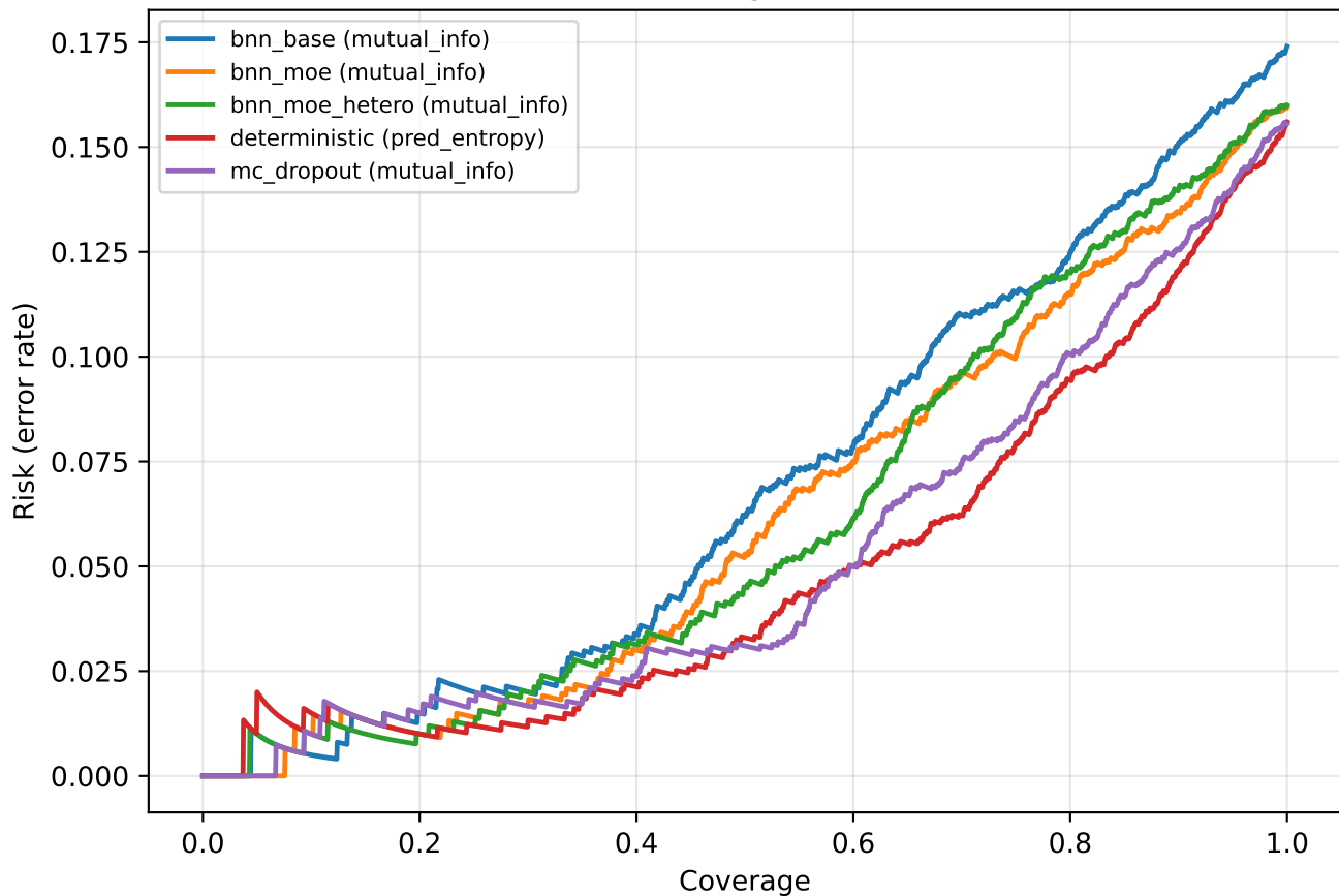
Risk-Coverage (test set)
