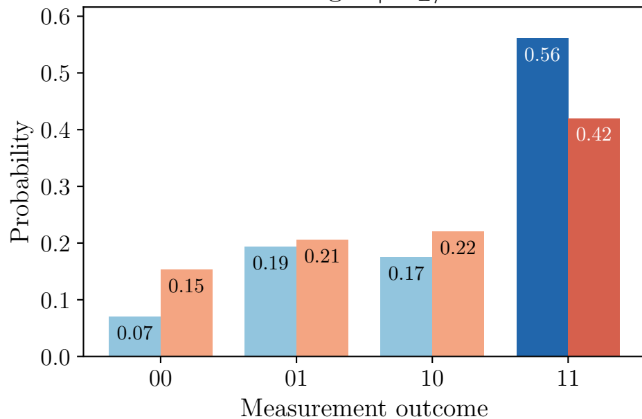
Target |11_L\rangle
