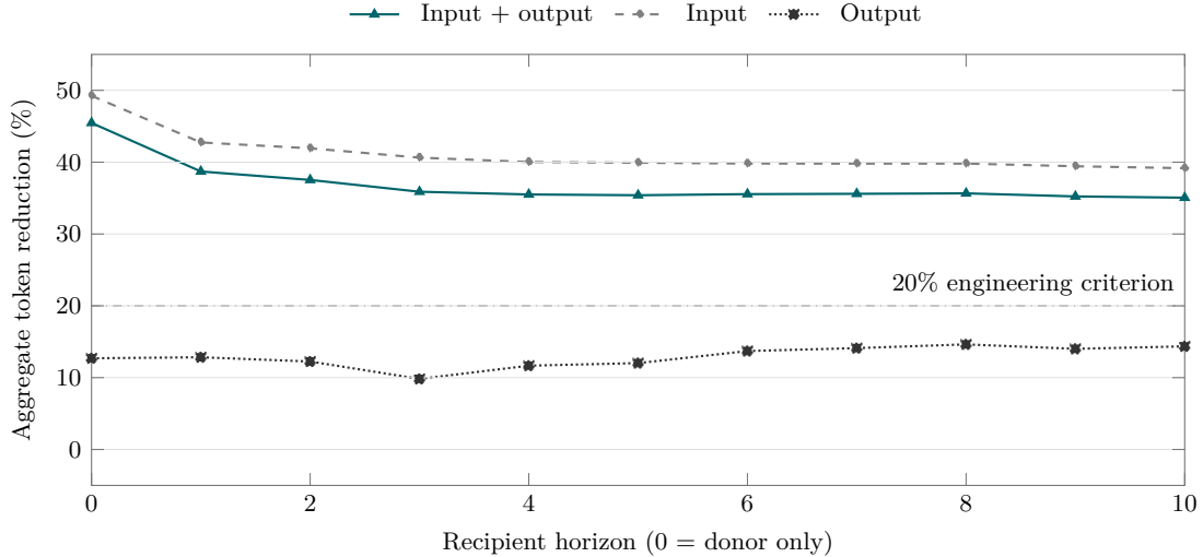
Figure 4: Observed aggregate token reductions as recipients accumulate, always including donors. Zero denotes donors alone. Input and output curves are components; the total curve uses their summed counts. The horizontal 20% reference is the frozen engineering criterion for the total at horizon ten. It is not a fitted effect, a cost threshold or a confidence limit.
