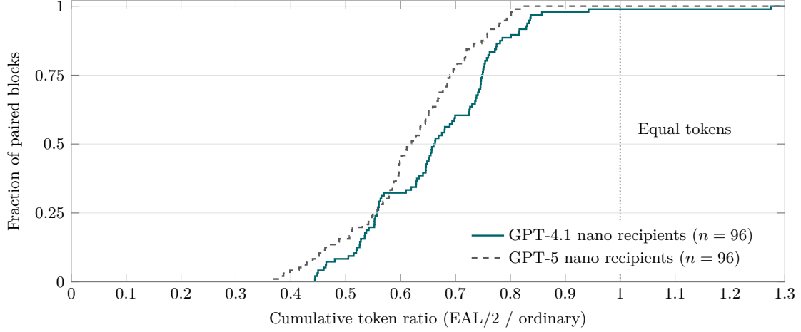
Figure 3: Empirical distributions of the paired cumulative token ratio, including donor and ten recipients. Each curve contains 96 paired blocks grouped by recipient model, pooling donor, task and tool settings. Ratios below one favour EAL/2. These are distributions of paired resource observations, not confidence distributions for the aggregate ratio.
