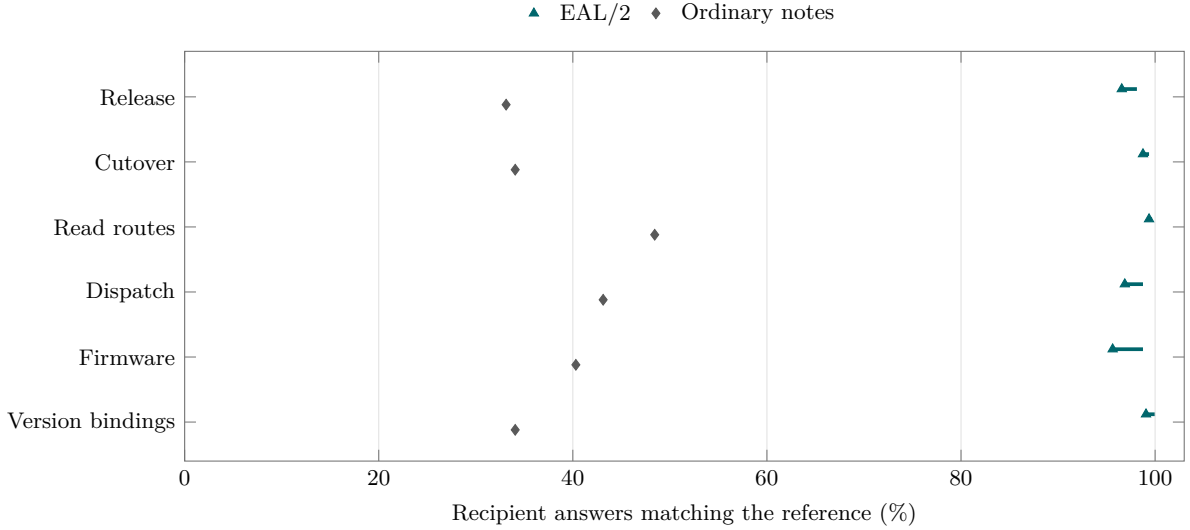
Figure 1: Decision-correctness envelopes for the six selected cases, pooling donor and recipient configurations. Markers show the lower endpoint; short horizontal segments extend to the upper endpoint when answers are ambiguous. Each marker represents 320 recipient answers nested within 32 sequences. The ranges express unresolved coding, not sampling precision.
