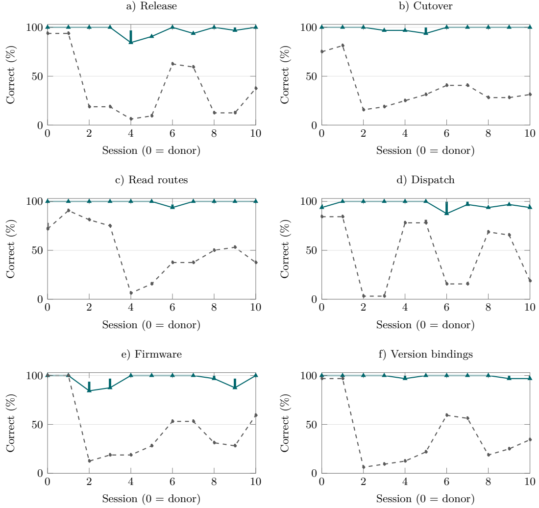
Figure 2: Correctness by task and session position. Solid teal triangles denote EAL/2 and dashed grey diamonds ordinary notes; vertical segments cover ambiguous coding. Each position contains 32 answers per arm. Position zero is the donor and is excluded from recipient correctness; positions one to ten are fresh recipients. The task fixtures change at even positions, with the next odd position retaining an eligible snapshot. The horizontal connections show ordered profiles, not independent observations or interpolation of task state.
