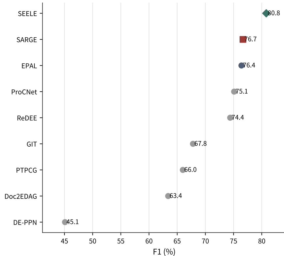
DuEE-Fin-dev500
