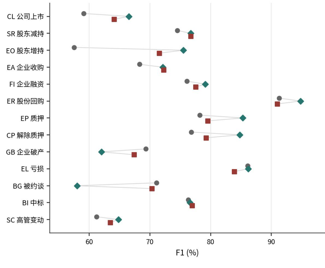
DuEE-Fin labeled test
