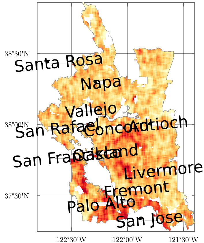
Nearest-hospital routing
