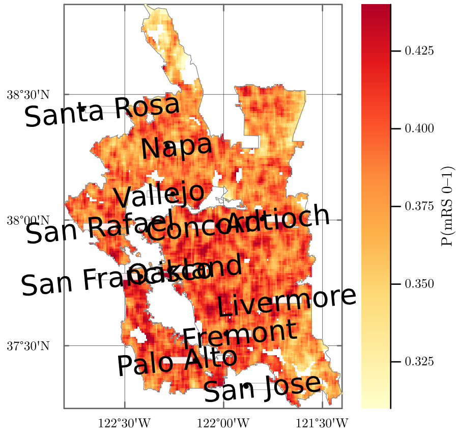
MDP policy
