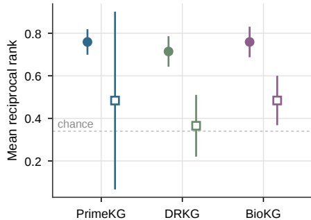
3 Performance splits on whether the graph contains the pair
