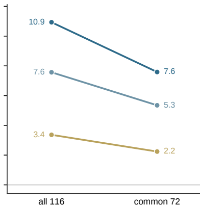
Gemini-3.1-Flash-Lite
