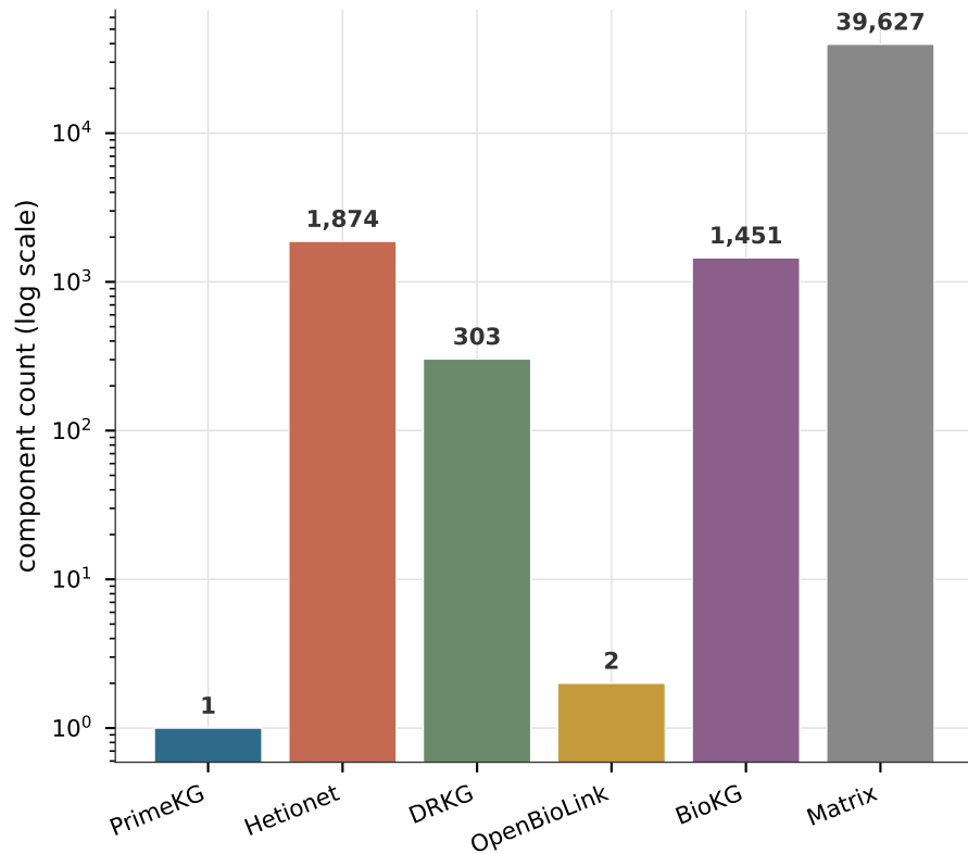
Connected components
