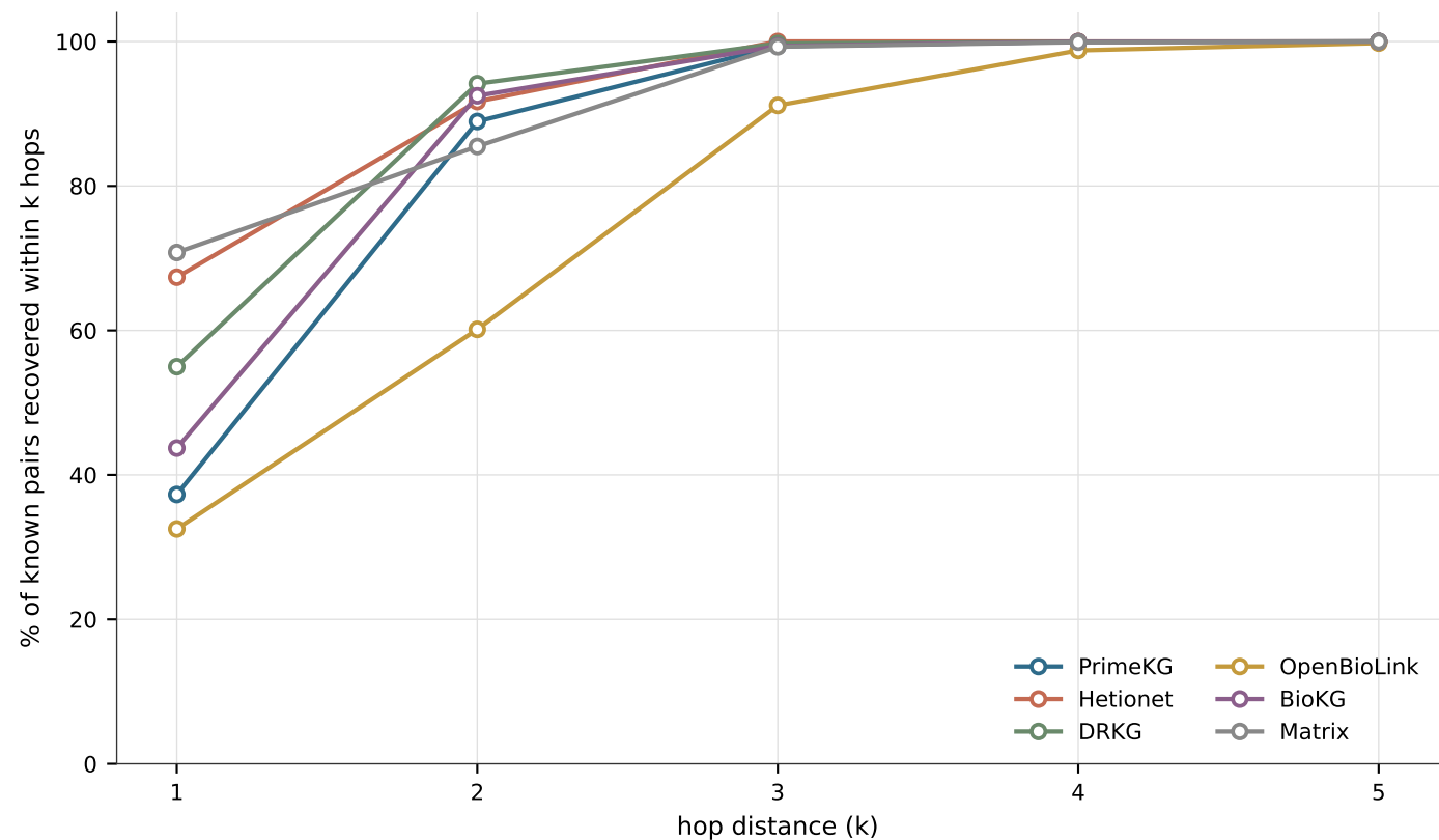
Known drug-disease pair recovery by hop distance
