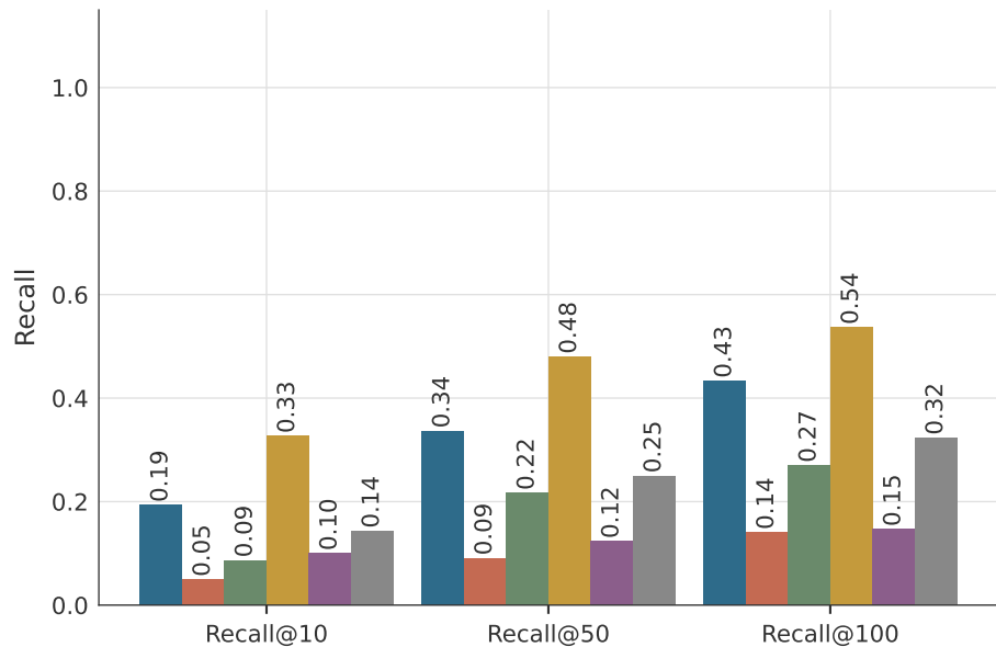
Recall Summary
