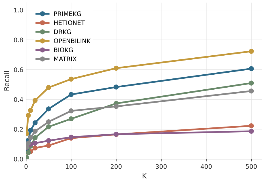
Recall@K
