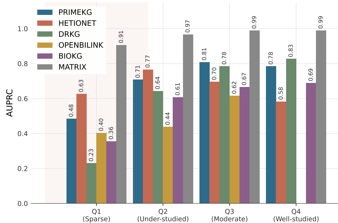
AUPRC by Disease Connectivity Tier
