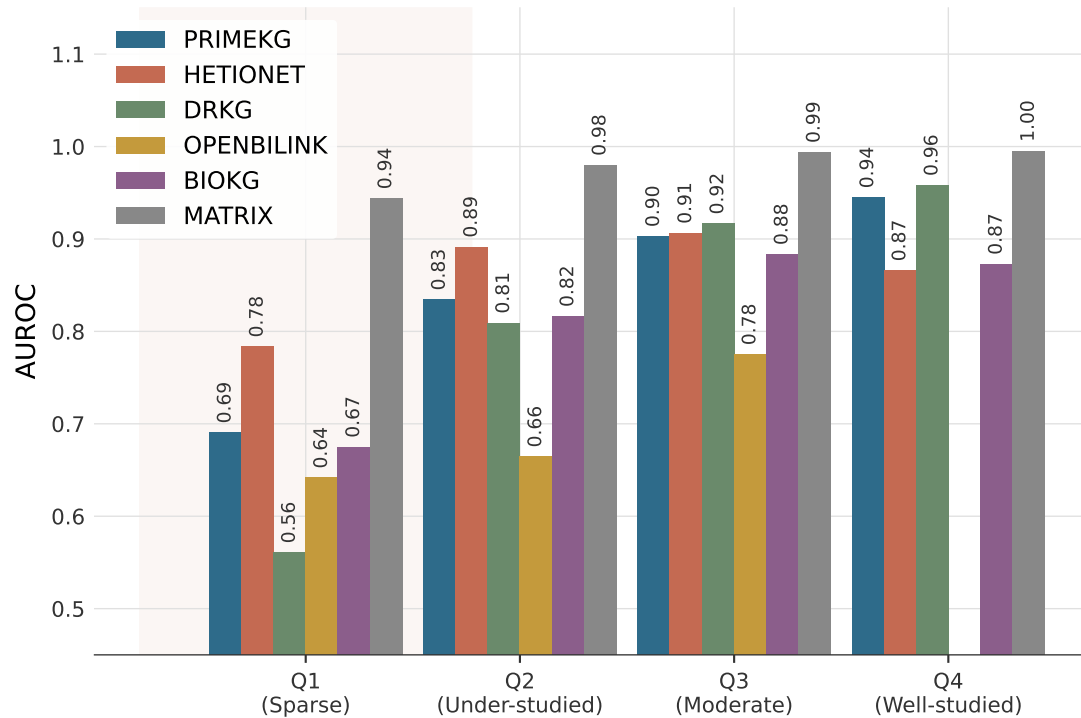
AUROC by Disease Connectivity Tier
