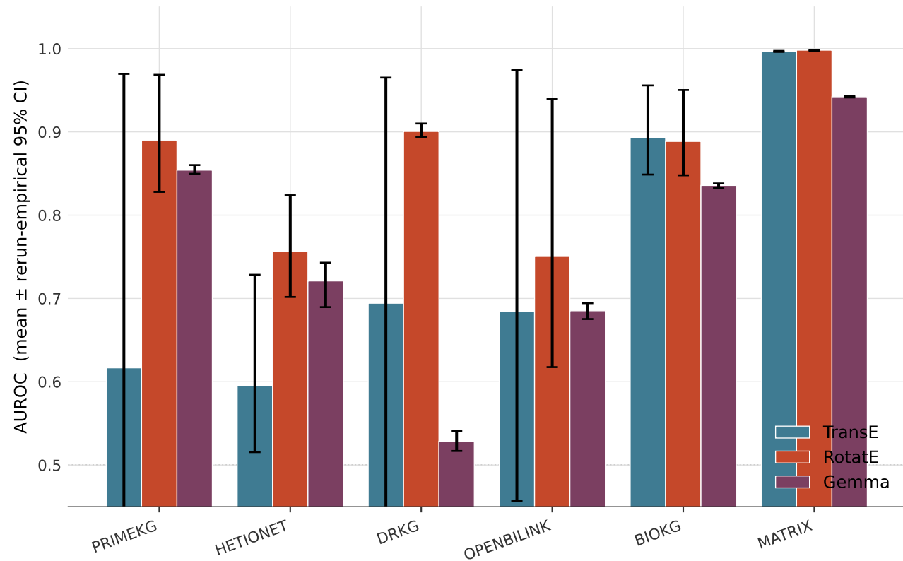
KG embedding performance with N=5 resampled reruns (type-constrained negatives)
