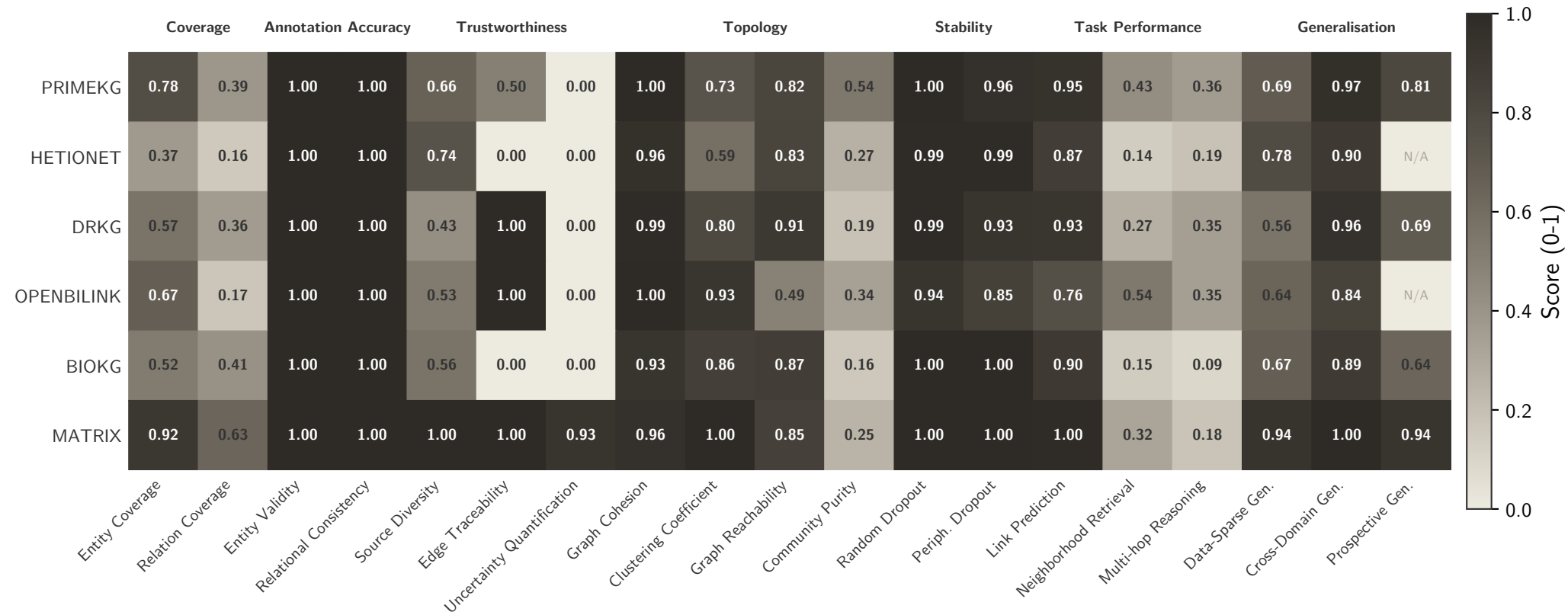
Metric performance across knowledge graphs
