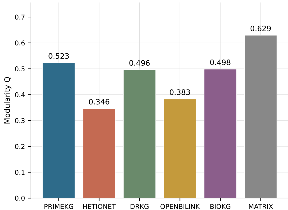
Louvain Modularity
