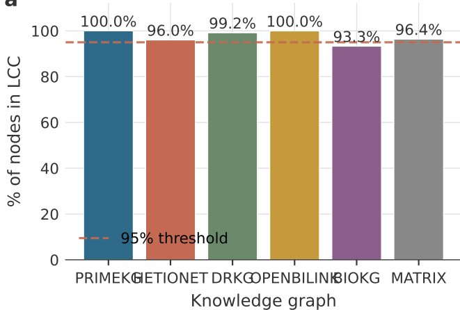
Largest Connected Component
