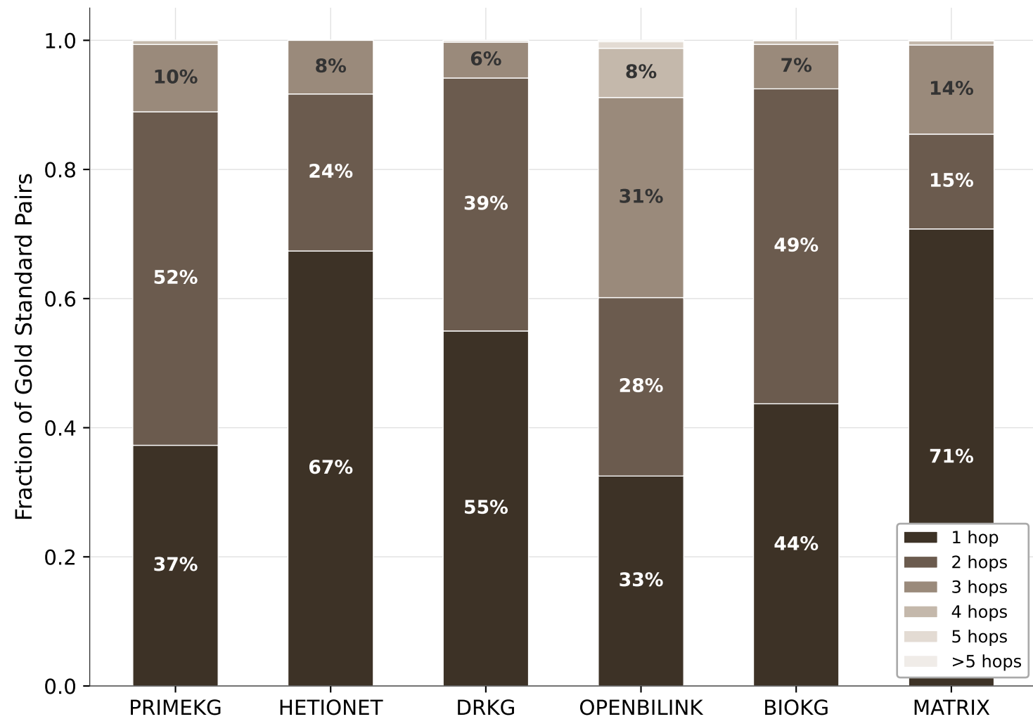
Hop Distance Distribution
