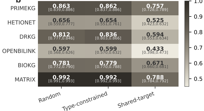
Link Prediction — AUPRC (Adamic-Adar)
