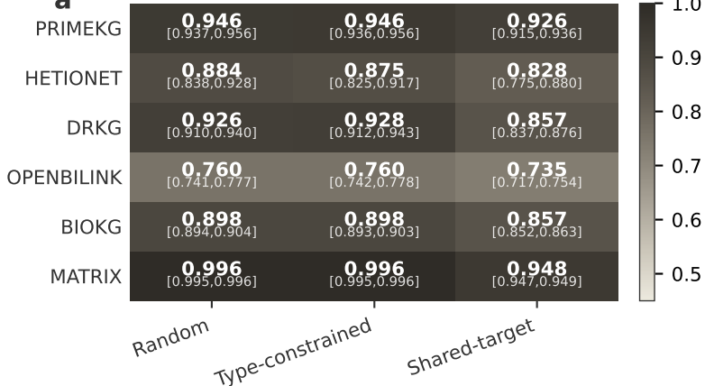
Link Prediction — AUROC (Adamic-Adar)
