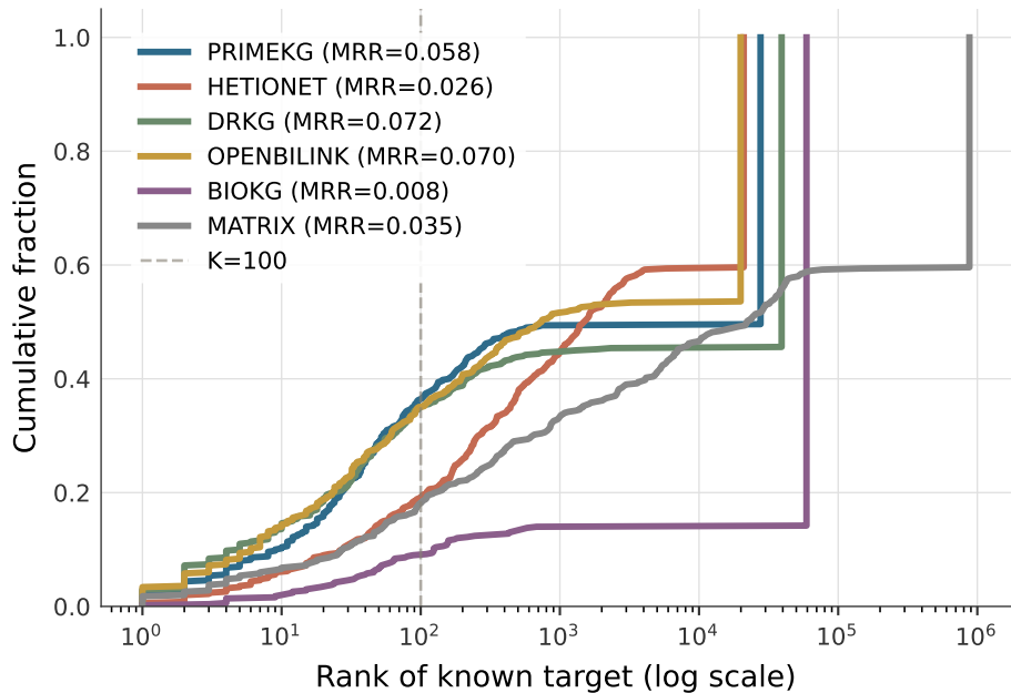
Target Rank CDF
