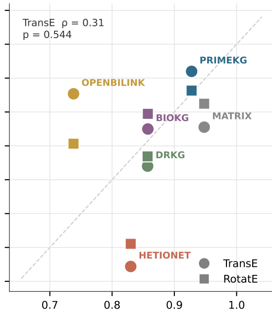
shared-target
