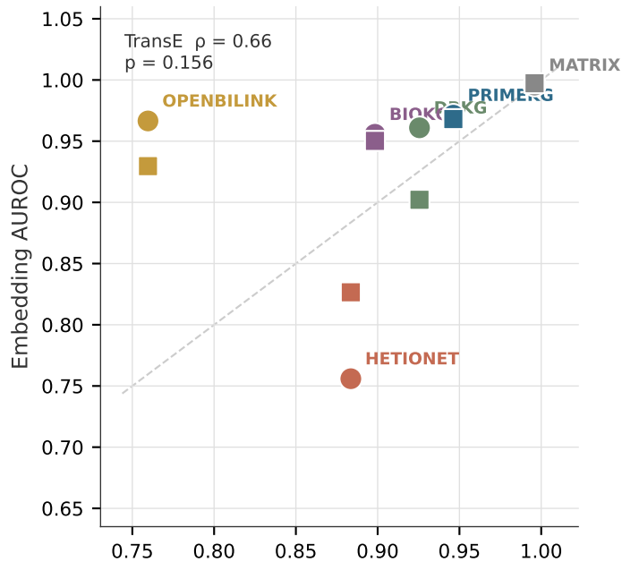
random
