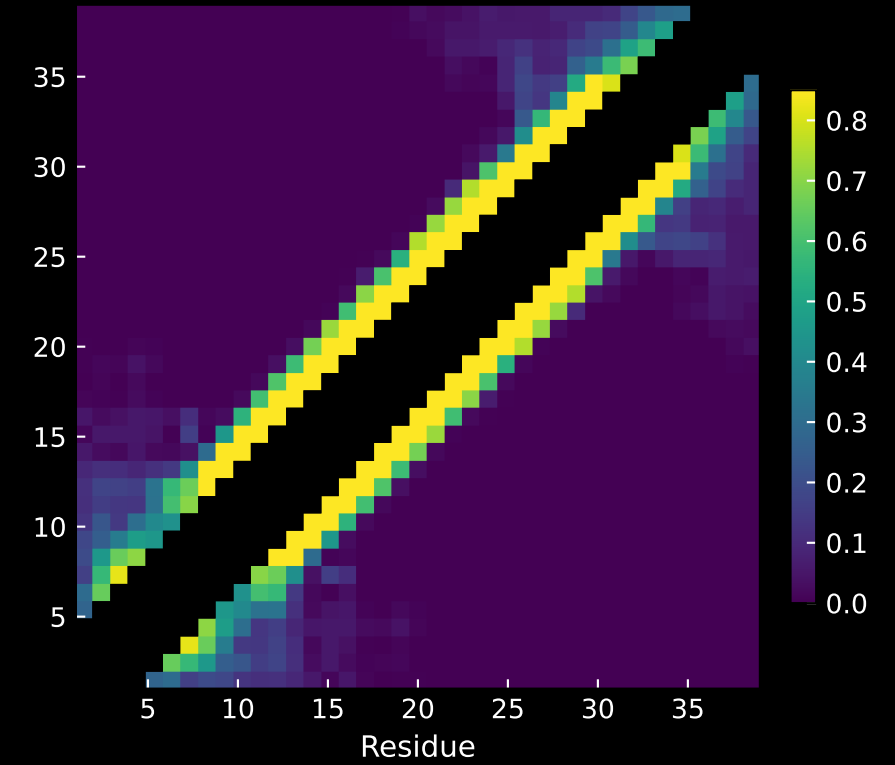
(F) G25D — Contact Frequency
