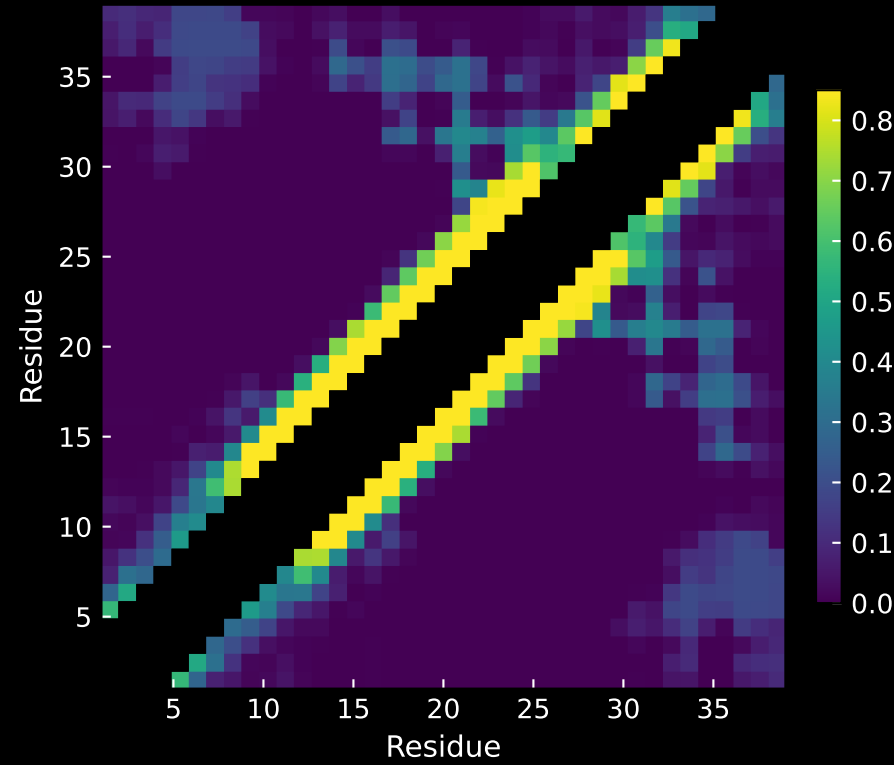
(E) WT — Contact Frequency
