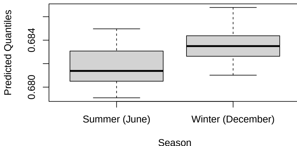
Boxplot of 50th Quantiles
