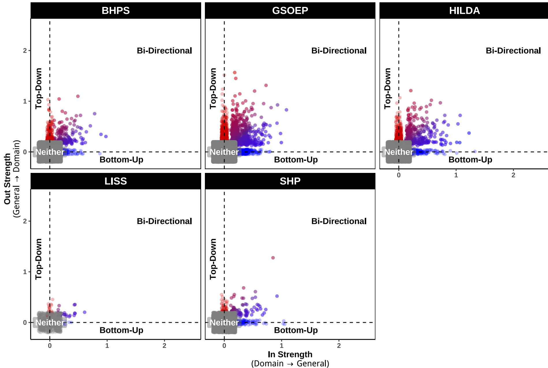
Scatterplot of participants with different patterns of random effects Thresholded at p < 0.2
