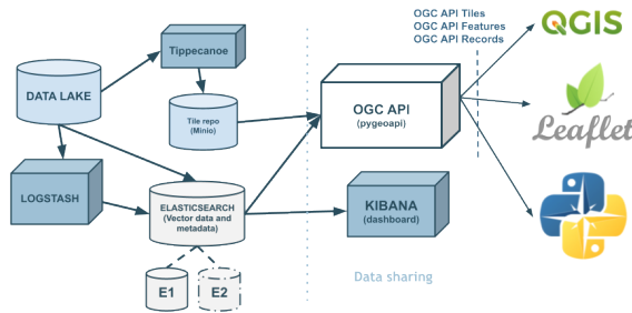
Figure 3. eMOTIONAL Cities SDI architecture
