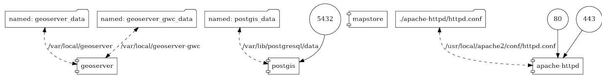
Figure 11. eMOTIONAL CITIES Legacy stack docker-compose structure
