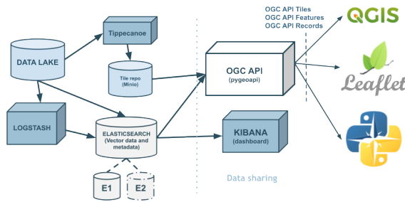
Figure 3. eMOTIONAL CITIES SDI architecture
