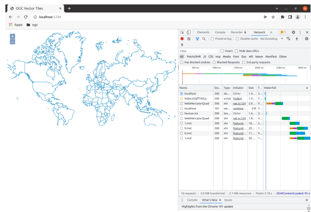
Figure 5. A basic implementation using OGC API - Tiles with OpenLayers
