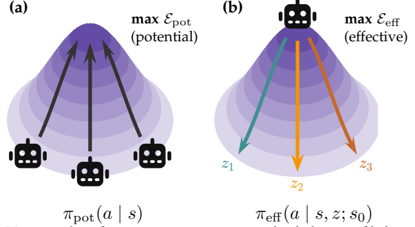
Two trained empowerment-maximizing policies characterize central states in an MDP. Consider an agent (robot) on a hill that is easier to descend than to ascend. (a) The potential policy ascends the empowerment landscape, using \mathcal{E}_{\text{pot}}(s) as an intrinsic reward. (b) The effective policy \pi_{\text{eff}} maximizes I^\pi(Z; S_+ | S_0) , associating each skill z with a downhill route.
