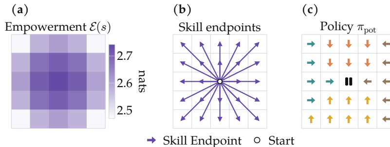
Figure 2: Skills measure the centrality of a state. (a) We visualize the potential empowerment field \mathcal{E}(s) for each state in a tabular GridWorld. The central state has high potential empowerment, because (b) the central state gives an agent access to a maximal set of distinguishable skills. (c) A potential empowerment policy ascends the potential empowerment landscape to the center state, from which it can execute different skills. See Theorem 4.1 for the formal statement, see Appendix K for tabular experiment details.
