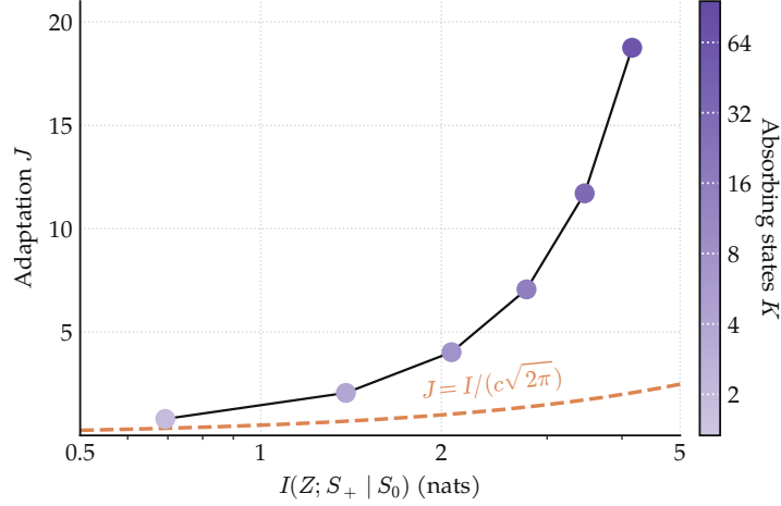
Figure 10: MI bound as a function of absorbing states (Theorem 4.3). Consider an MDP with one starting state and K absorbing target states. Each of the K actions transitions deterministically to a distinct target. We normalize occupancies over the targets (neglecting the occupancy of the starting state). Thus, K counts the maximum possible number of total skills. The scaled MI (orange) correctly lower bounds the adaptation J (purple). The bound weakens as the number of absorbing target states in the MDP grows.
