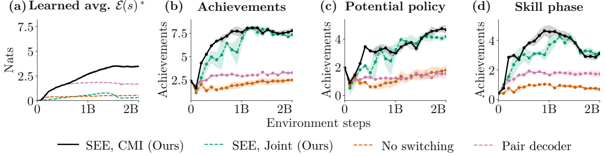
Figure 10: Craftax-Classic ablations (CMI SEE: 5 seeds; each ablation: 3). The black curve is the SEE with the CMI classifier (Ours). The ablations are SEE with Joint MI (Ours), no switching (25% potential-policy episodes during training), and pair decoder. (a) Learned empowerment estimates rise over training for the base method. (b) Total achievements per rollout. (c) Achievements in the first 100 potential-policy actions. (d) New achievements in the subsequent skill phase of up to 900 actions. All methods use 128 fresh worlds and skills per seed and evaluation checkpoint. Curves show mean \pm standard error across training seeds, with per-seed EMA ( \alpha = 0.05 ) only in (a). Achievement panels are unsmoothed and display every tenth evaluation checkpoint plus the final checkpoint.
