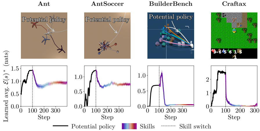
Figure 4: Potential empowerment policies accrue empowerment, while skills spend it. (Top row) Over the course of the trajectory, the potential empowerment policies “gather” empowerment, reaching empowered states. Correspondingly, the empowerment estimates increase over the course of the trajectory. (Bottom row) At the gray skill switch mark, executing a skill from the reached state “spends” the empowerment, reflecting the intuition that potential empowerment policies collect power and effective empowerment spends power. Traces use one seed and 30 skills per environment.
