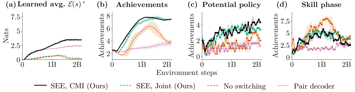
Figure 10: Crafttax-Classic ablations (3 seeds; Joint MI: 5). The black curve is the SEE with the CMI classifier (Ours). The ablations are SEE with Joint MI (Ours), no switching (25% potential-policy episodes), and pair decoder. (a) Learned empowerment estimates rise over training for the base method. (b) Achievements per rollout. (c) New achievements in 100 potential-policy actions, using one rollout per seed/checkpoint for every method. (d) New skill-phase achievements from four branches per seed/checkpoint; no-switching skills start from reset. Curves show mean \pm standard error, with per-seed EMA ( \alpha = 0.05 ) in (a,b) and unsmoothed checkpoints in (c,d).
