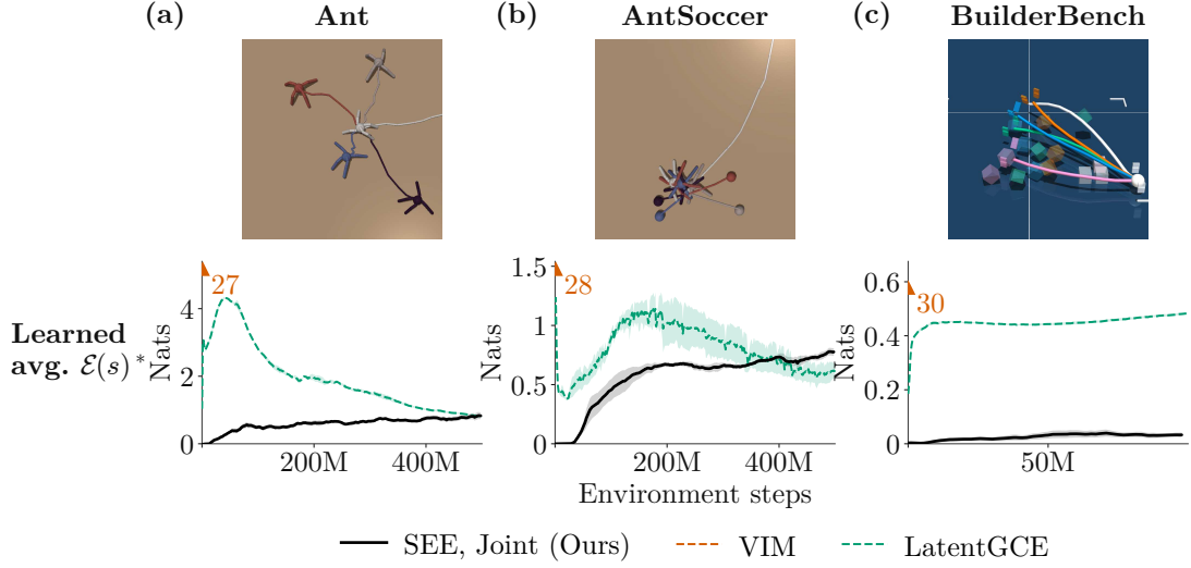
Figure 8: Learned empowerment in continuous settings. SEE (Black) empowerment values gradually increase over time. Meanwhile, VIM (Orange) and LatentGCE (Green) empowerment values are unstable. *As a note, learned estimates use different objectives and regularization, so their magnitudes are not directly comparable across methods. Five seeds for SEE; three per baseline.
