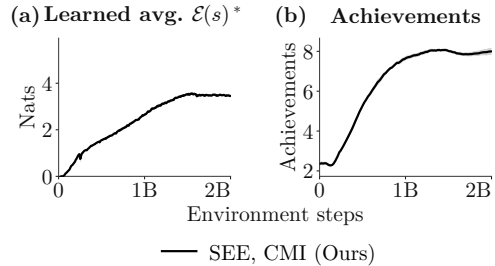
Figure 1: The potential empowerment estimate increases with control in Crafter. (a) The learned empowerment estimate increases consistently. (b) Simultaneously, the agent intrinsically learns to complete achievements in the environment without access to external rewards . Curves show mean \pm standard error across three seeds.
