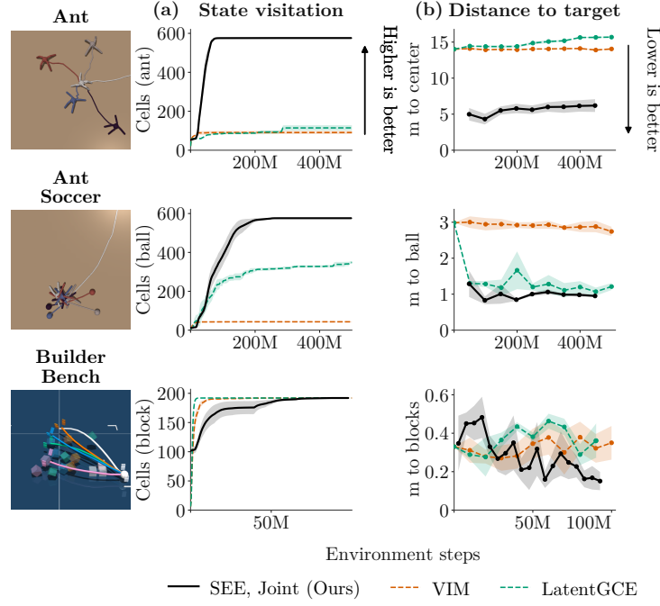
Figure 3: Potential empowerment and control increases over training (continuous settings). We compare SEE (Black) and baselines VIM (Orange) and LatentGCE (Green). (a) Only SEE visits diverse states across these environments, which is necessary to learn correct models and decoders of dynamics and skills. (b) SEE consistently learns potential empowerment policies that navigate to central regions in Ant, to the ball in AntSoccer, and to the blocks in BuilderBench. VIM is unstable and largely stationary in Ant and AntSoccer. LatentGCE is also stationary in Ant, and generally does not reach the blocks and soccer ball in the other environments as consistently as SEE. Five seeds for SEE; three per baseline.
