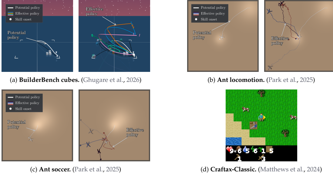
Figure 2: Empowerment-maximizing behavior across environments. (a) In the BuilderBench task, a gripper interacts with blocks in an open-ended setting. The potential empowerment policy is visualized with the white rollout, navigating to the blocks and staying there. Then, the effective empowerment policies, or skills, knock the blocks in different directions (colorful lines and blocks). (b) In the first version of the AntSoccer task, an agent can be empowered without interacting with the ball. The potential empowerment policy (white) navigates to the central area of the arena, while the skills branch out from this point. (c) In the second version of the AntSoccer task, an agent can only be empowered if it controls the ball. The trained potential empowerment policy reaches the soccer ball, while skills kick the soccer ball in different directions. (d) In Craftax-Classic, the potential empowerment agent gathers materials, builds a crafting table, then builds tools using gathered materials. One seed per environment.
