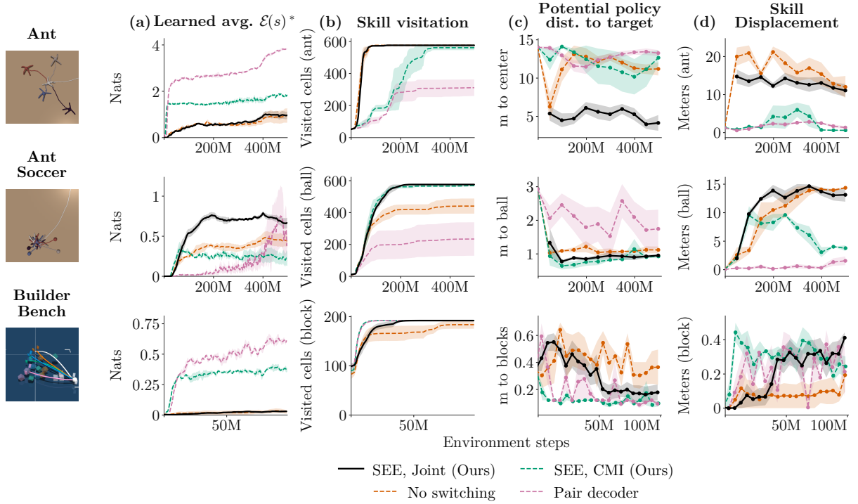
Figure 9: We compare the full method with variants that remove the two-phase rollout (no switching, orange), replace joint MI with conditional MI (green), or replace the bilinear logit with a general MLP (pair decoder, pink). The solid black curve shows SEE, and the colored dashed curves show the ablations. (a) For all methods, average empowerment increases over training. * Learned empowerment estimates use different objectives and regularization, so their magnitudes are not directly comparable across methods. (b) The skill visitation of SEE quickly saturates for these environments. Meanwhile, the ablations struggle to get visitation in a subset of the different environments. (c) SEE consistently learns potential policies that reach the center of the arena (Ant), approach the ball (AntSoccer), and reach the blocks (BuilderBench). While all variants successfully learn to reach the blocks in BuilderBench, the ablations all struggle to reach the center of the arena in Ant and some struggle to reach the ball in AntSoccer. (d) SEE consistently learns effective policies with large displacements. Five seeds for SEE; three per ablation.
